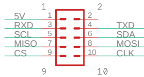
WIPHONE_DAUGHTERBOARD
